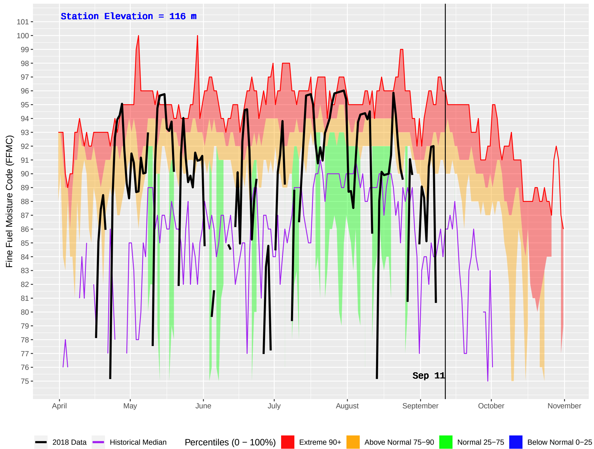
SCAR CREEK (82) : Historical (1982–2016) and Current (2018) Daily Fine Fuel Moisture Code (FFMC)
